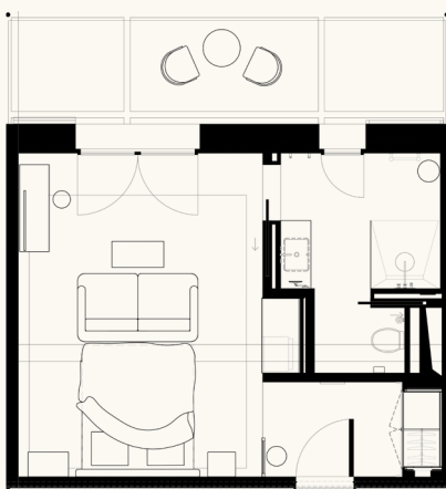
PLAN 2
