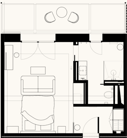
PLAN 2
